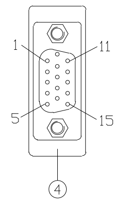
HD15 FEMALE INSULATOR:BLACK
