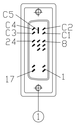
DVI(12+5) MALE INSULATOR:BLACK
